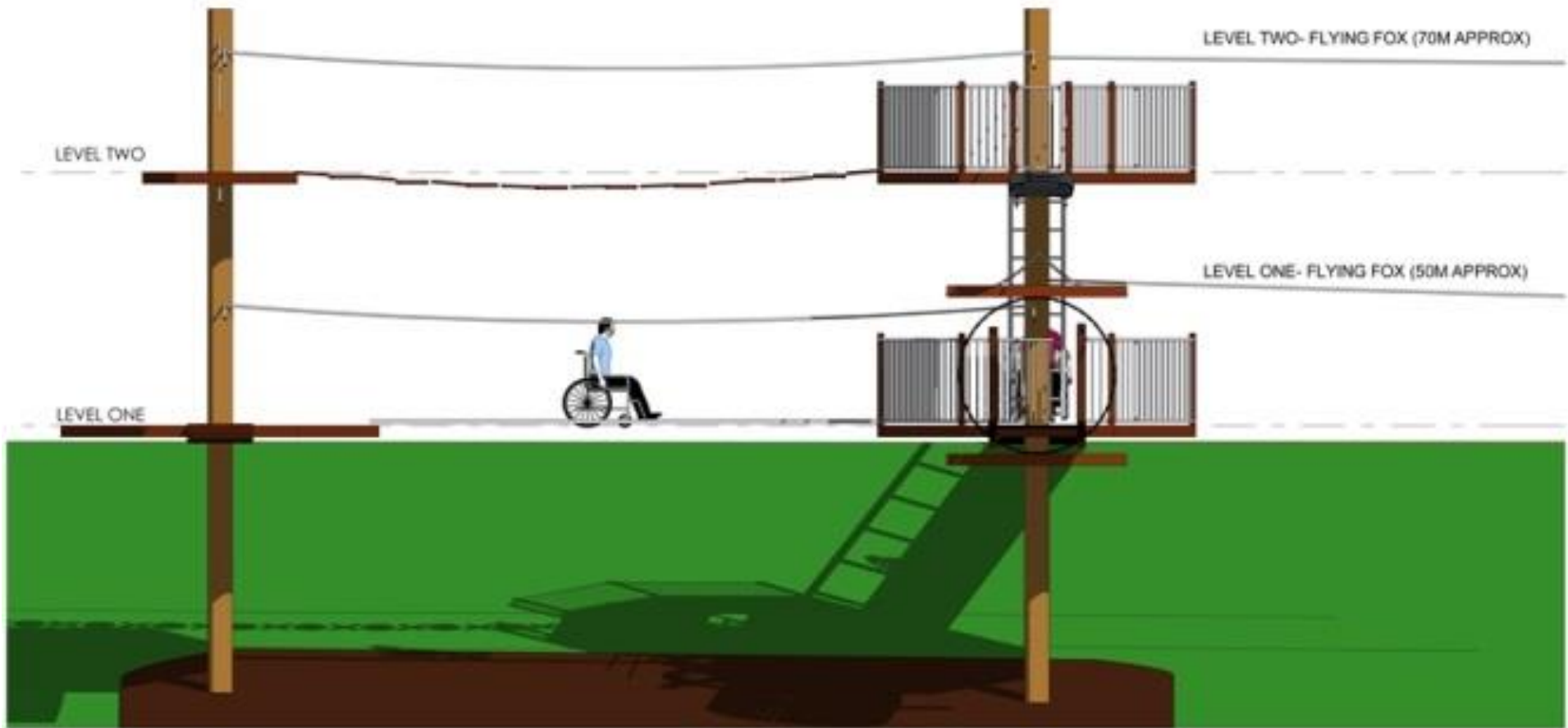
SECTION A
